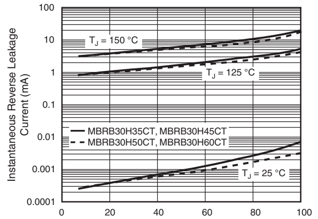
Fig. 4 - Typical Reverse Characteristics Per Diode
