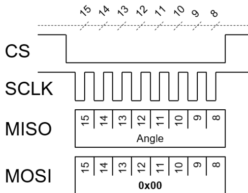
Figure 10: Partial 8-Bit SPI Angle Reading Diagram
