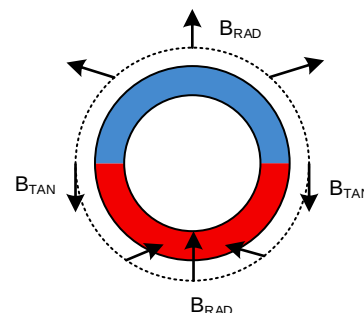
Figure 20: Side-Shaft Field
