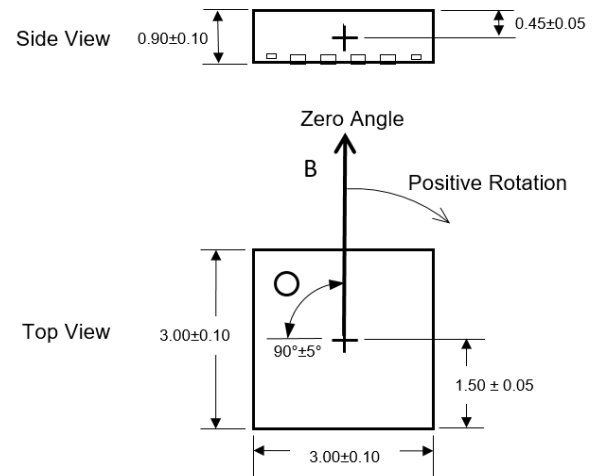
Figure 3: Detection Point and Default Positive Direction
