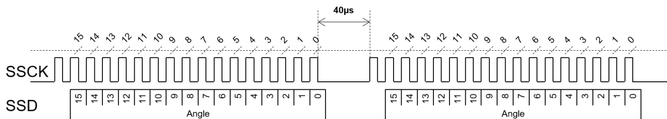
Figure 17: Diagram of Two Consecutive 16-Bit SSI Angle Readings with the Required Dead Time between the Frames
