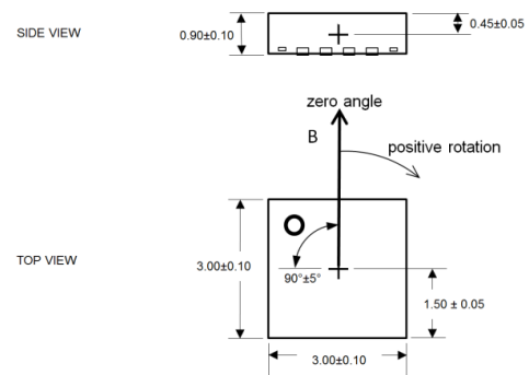
Figure 3: Detection Point and Default Positive Direction
