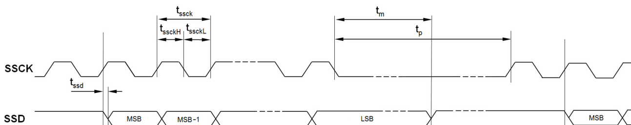
Figure 15: SSI Timing
