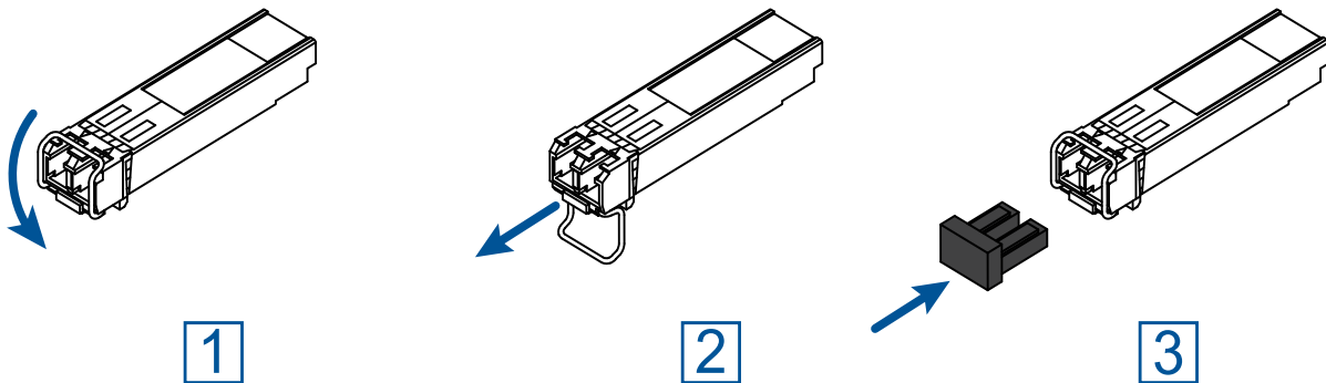
Figure 16: De-installing SFP transceivers: De-installation sequence
