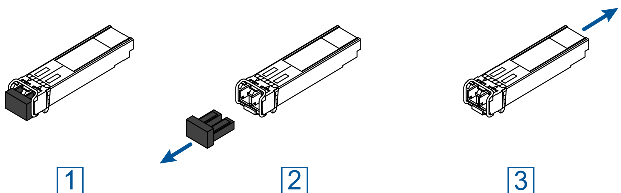
Figure 10: Installing SFP transceivers: Installation sequence
