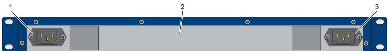
Figure 5: MACH104-20TX-FR... connections on the back of the device 1 - Standard power supply 100 V AC ... 240 V AC 2 - MACH104-20TX-FR... device 3 - Redundant power supply 100 V AC ... 240 V AC
