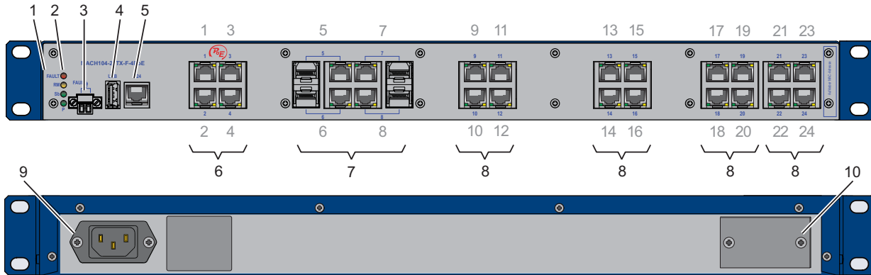
Figure 3: Overview over interfaces, display and operating elements of the MACH104-20TX-F-4-PoE...
