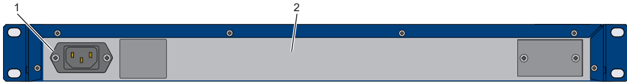
Figure 6: MACH104-20TX-F-4-PoE... connections on the back of the device 1 - Standard power supply 100 V AC ... 240 V AC 2 - MACH104-20TX-F-4-PoE... device
