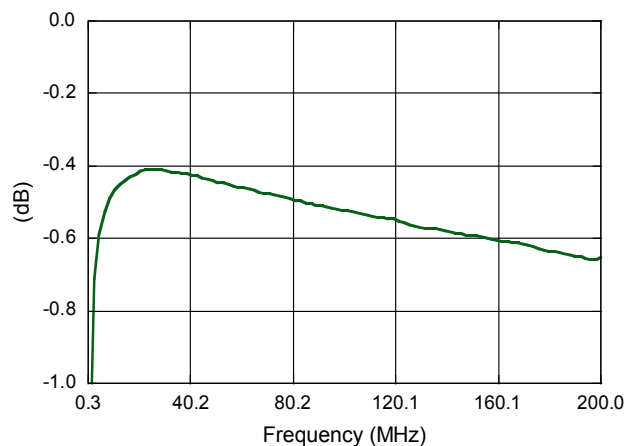
Insertion Loss (pin 4_1)
