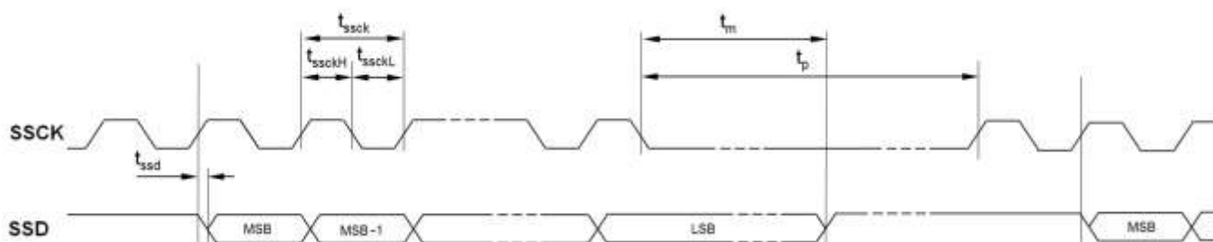
Figure 15: SSI Timing
