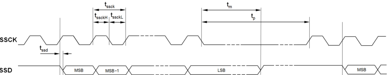
Figure 15: SSI Timing
