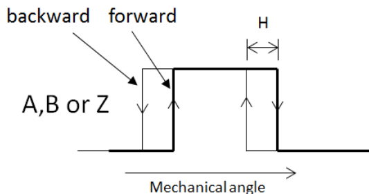
Figure 27: Hysteresis of the Incremental Output
