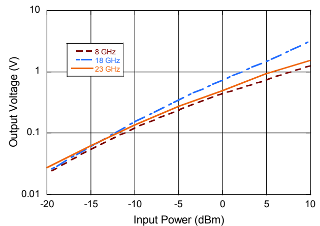
Output Voltage vs. Input Power
