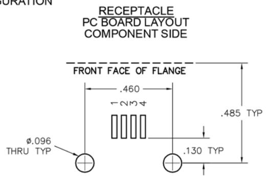
FOOTPRINT/PAD CONFIGURATION
