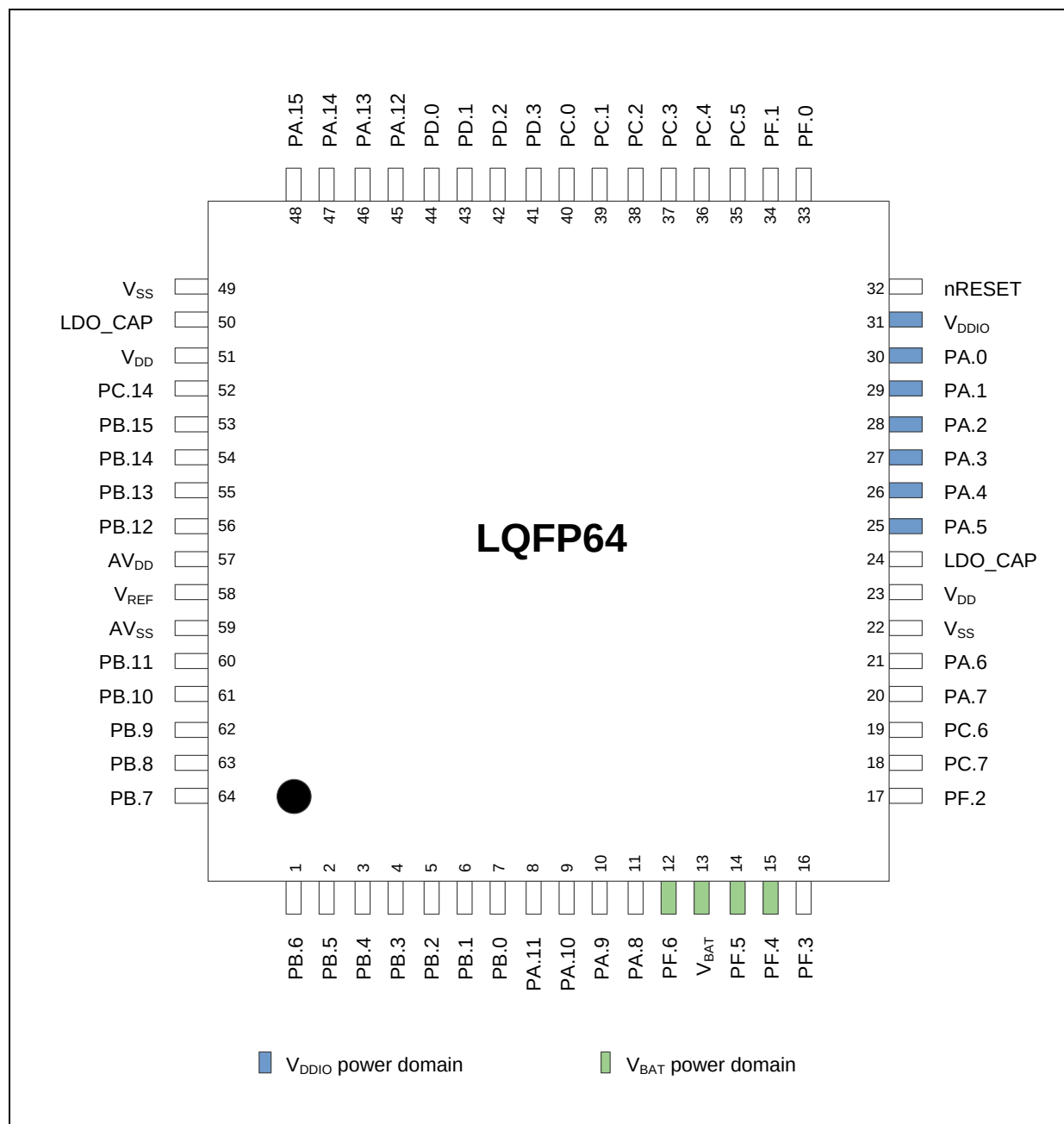
Figure 4.1-4 LQFP-64 Pin Diagram (0/1 USB FS with V_{BAT} )
