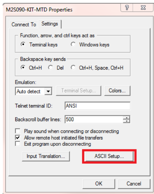
Figure 34 Settings Tab
