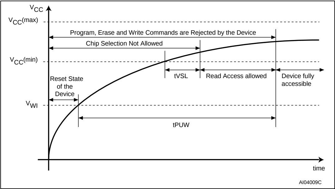
Figure 21. Power-up timing
