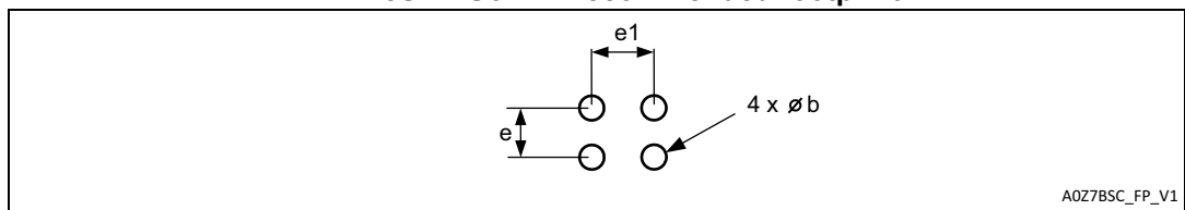
Figure 15. WLCSP package with Back Side Coating (BSC) M24128S-FCU6T/TF recommended footprint
