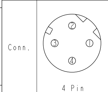
Pin Assignments Front View \triangle B
