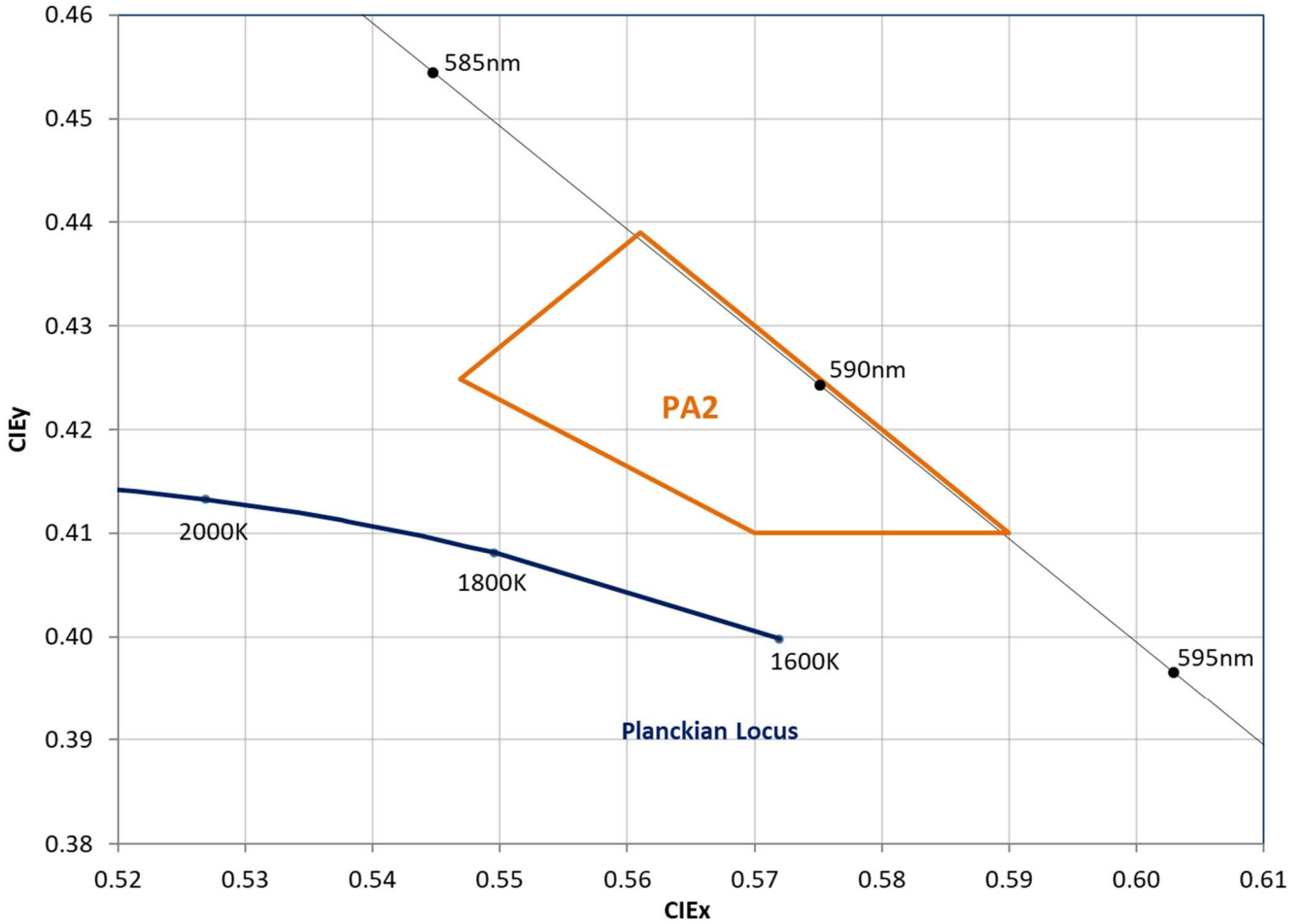
Standard Chromaticity Groups plotted on excerpt from the CIE 1931 (2°) x-y Chromaticity Diagram
