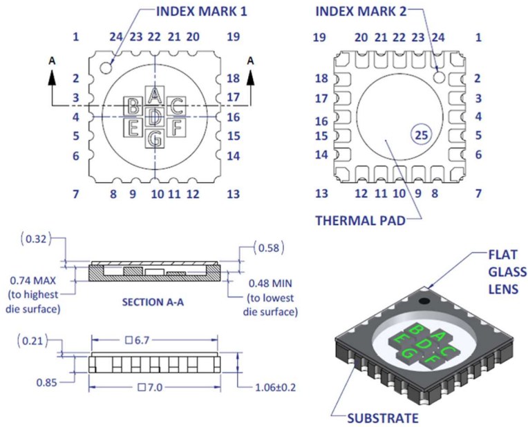
Figure 1: Package Outline Drawing
