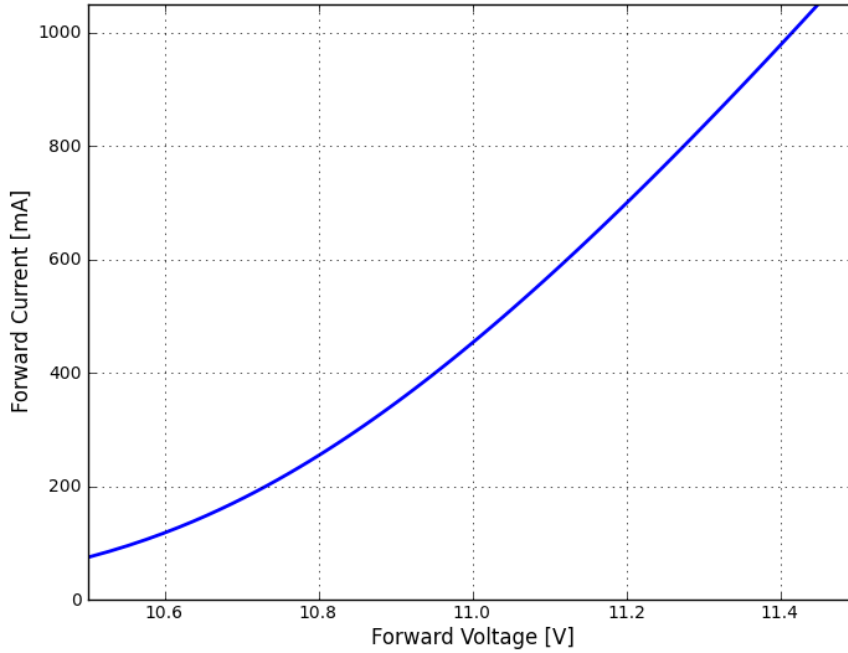
Figure 13. Forward current vs. forward voltage (12V).
