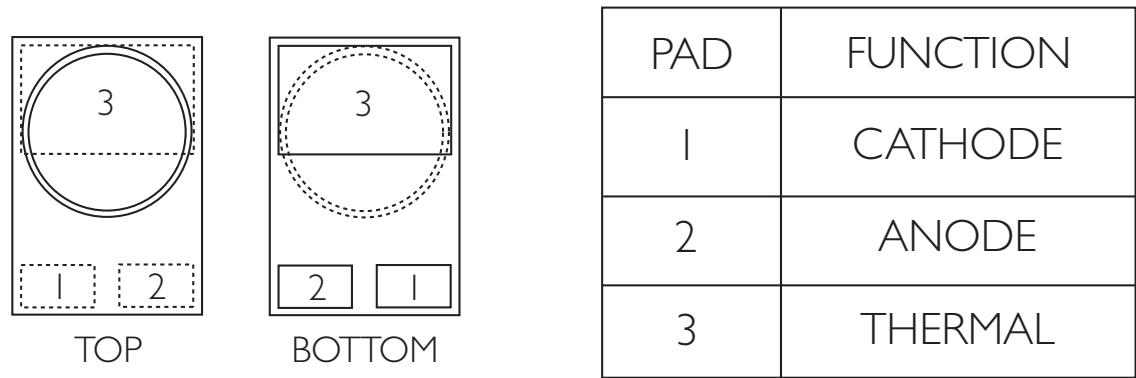
Figure 2. Pad configuration.
