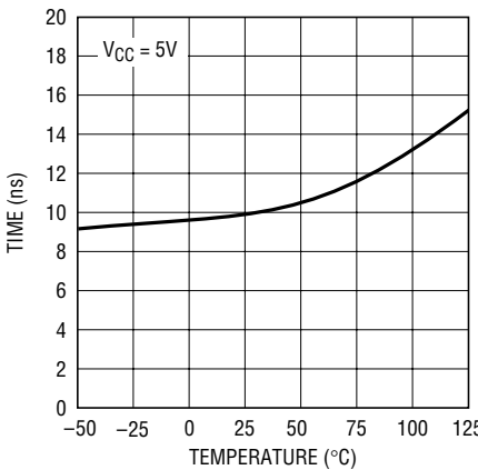
RS485 Receiver Skew |t_{PLH} - t_{PHL}| vs Temperature
