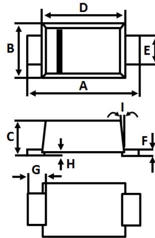
DO-219AA
