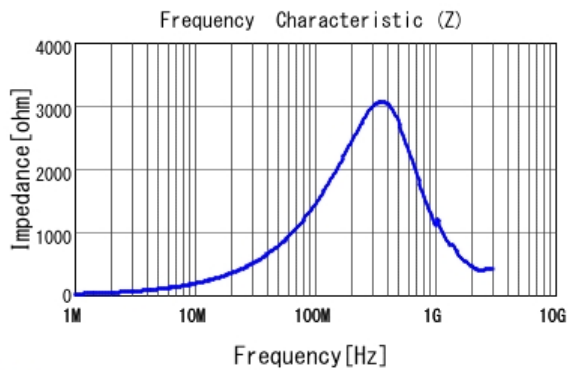
■ LQW32FT3R3M0H |Z|
