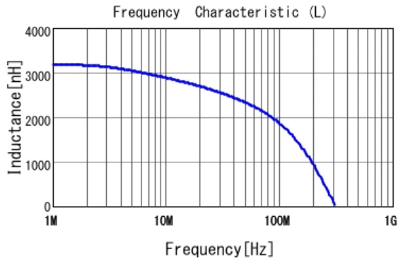
■ LQW32FT3R3M0H L
