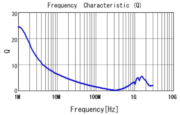
■ LQW32FT3R3M0H Q
