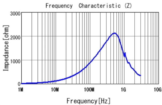
■ LQW32FT2R2M0H |Z|
