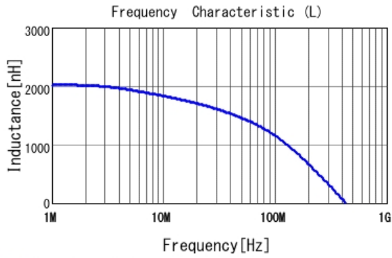
■ LQW32FT2R2M0H L
