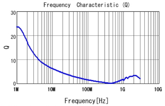
■ LQW32FT2R2M0H Q
