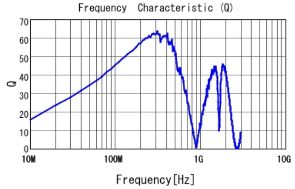
■ LQW2BASR27G00 Q
