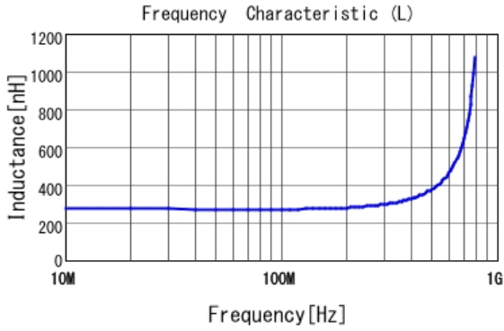
■ LQW2BASR27G00 L
