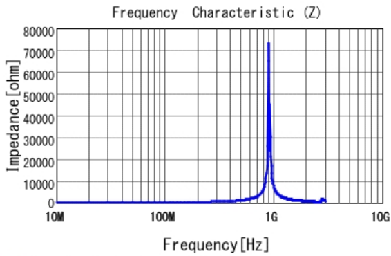
■ LQW2BASR27G00 |Z|
