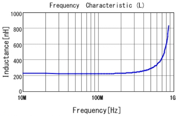
■ LQW2BASR22G00 L
