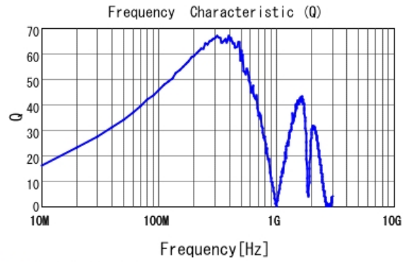
■ LQW2BASR22G00 Q
