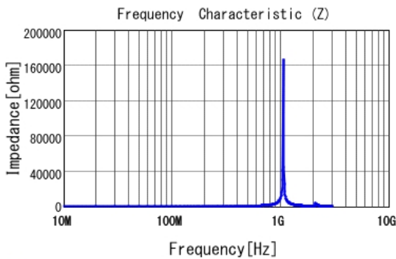
■ LQW2BASR18G00 |Z|
