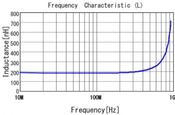
■ LQW2BASR18G00 L
