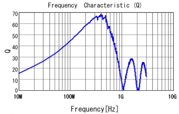
■ LQW2BASR18G00 Q
