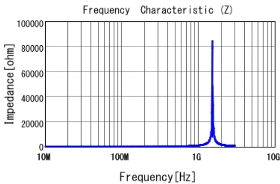
■ LQW2BASR10G00 |Z|
