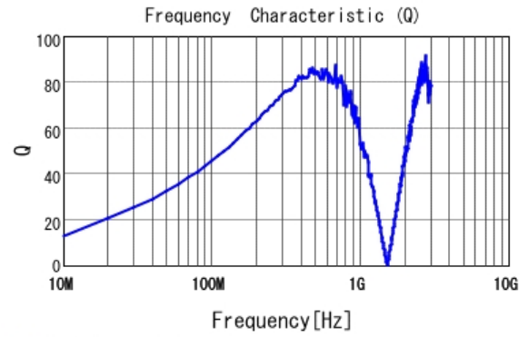
■ LQW2BASR10G00 Q
