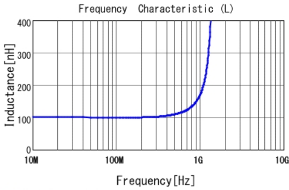
■ LQW2BASR10G00 L
