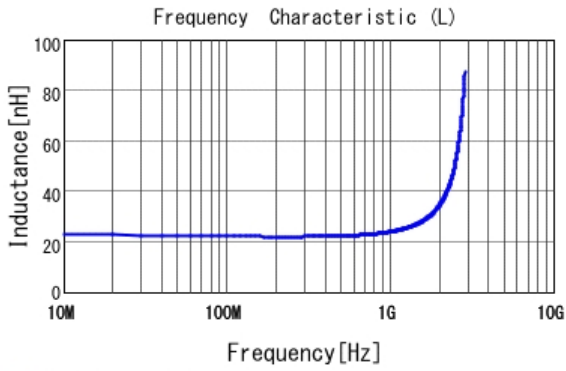
■ LQW2BAS22NG00 L
