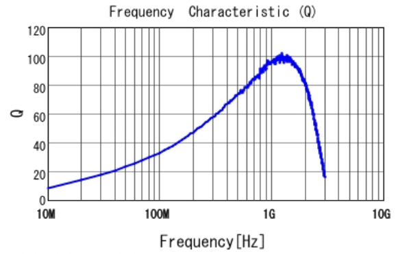
■ LQW2BAS22NG00 Q
