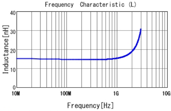
■ LQW2BAS15NG00 L
