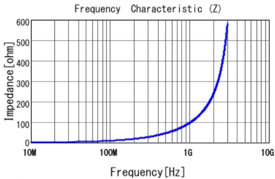
■ LQW2BAS15NG00 |Z|
