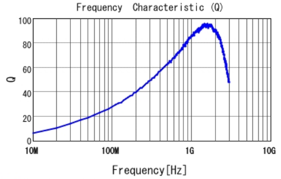
■ LQW2BAS15NG00 Q
