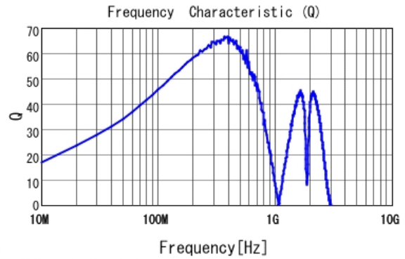
■ LQW2BANR20G00 Q
