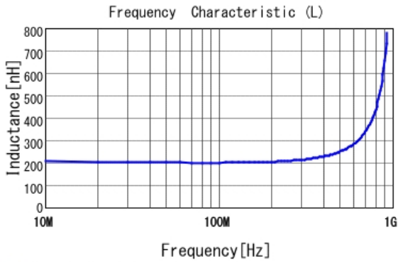
■ LQW2BANR20G00 L
