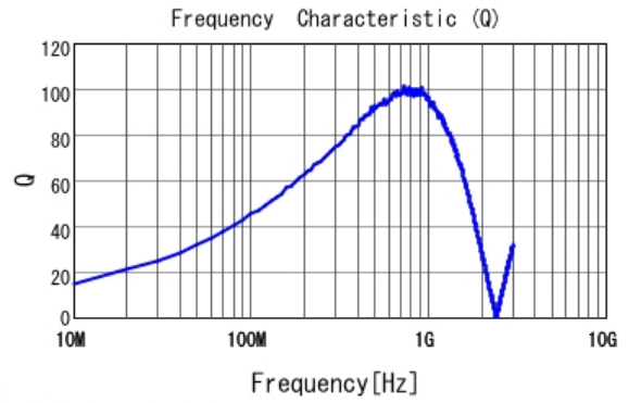
■ LQW2BAN33NJ00 Q
