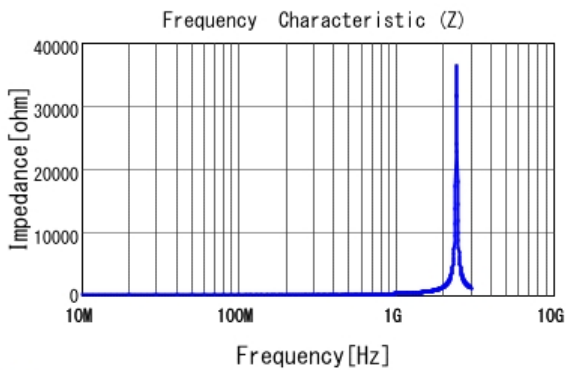
■ LQW2BAN33NJ00 |Z|
