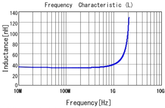
■ LQW2BAN33NJ00 L
