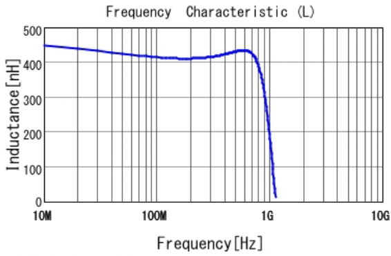
■ LQW15CAR43J00 L
