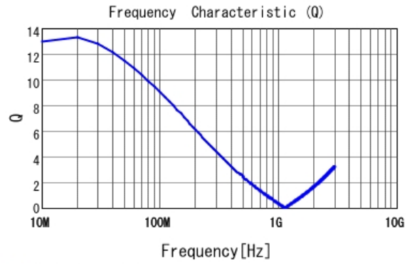
■ LQW15CAR43J00 Q
