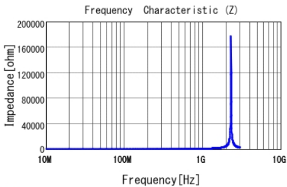
■ LQW15AWR10G80 |Z|
