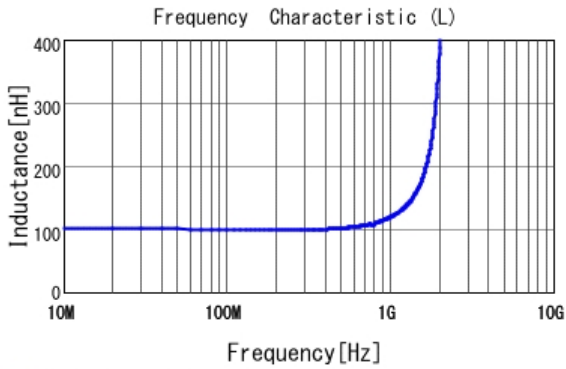
■ LQW15AWR10G80 L
