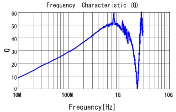
■ LQW15AWR10G80 Q
