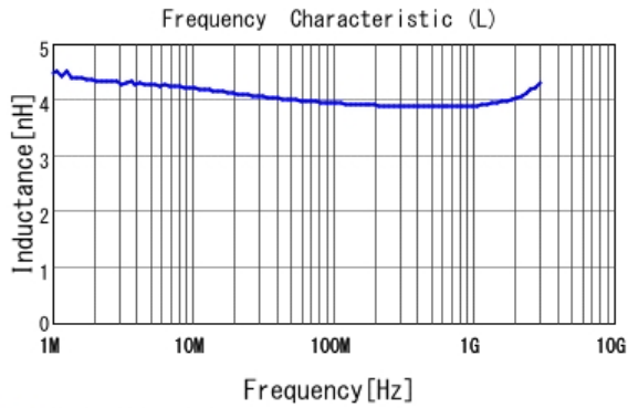
■ LQW15AN4N0G80 L
