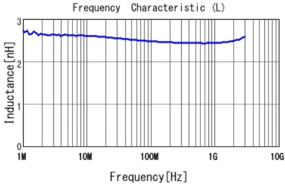
■ LQW15AN2N5B8Z L
