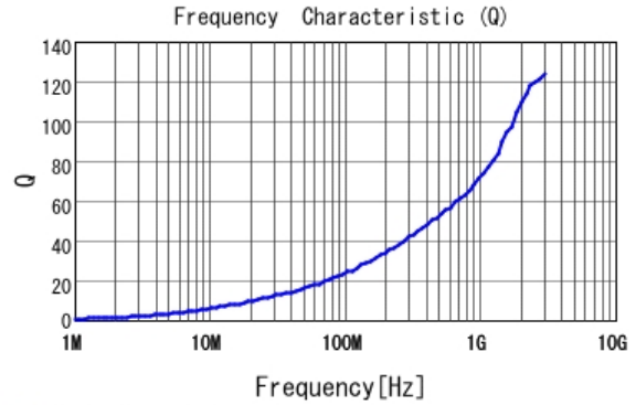
■ LQW15AN2N5B8Z Q
