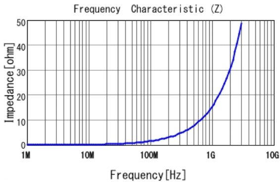
■ LQW15AN2N5B8Z |Z|
