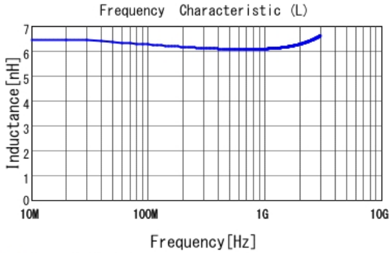
■ LQW04AN6N2D00 L
