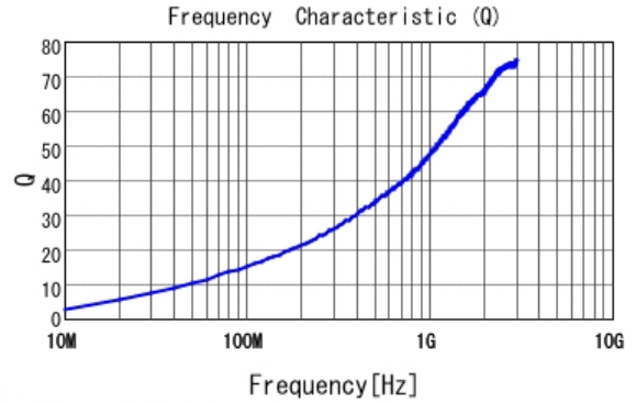
■ LQW04AN6N2D00 Q
