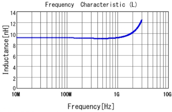
■ LQP15MN9N1B02 L
