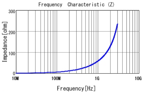
■ LQP15MN9N1B02 |Z|
