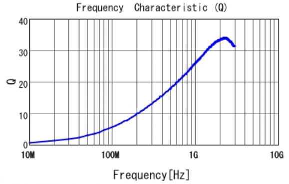
■ LQP15MN9N1B02 Q
