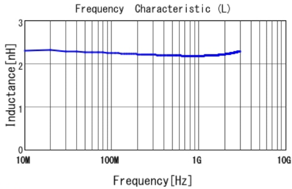
■ LQP15MN2N2W02 L
