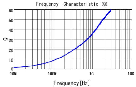
■ LQP15MN2N2W02 Q
