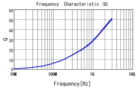
■ LQP15MN1N6W02 Q
