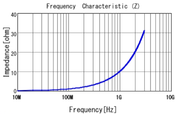
■ LQP15MN1N6W02 |Z|
