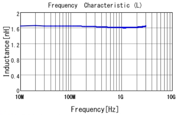
■ LQP15MN1N6W02 L
