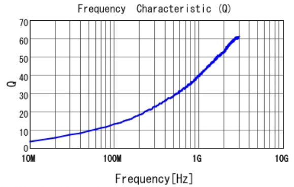
■ LQP03TQ3N0B02 Q
