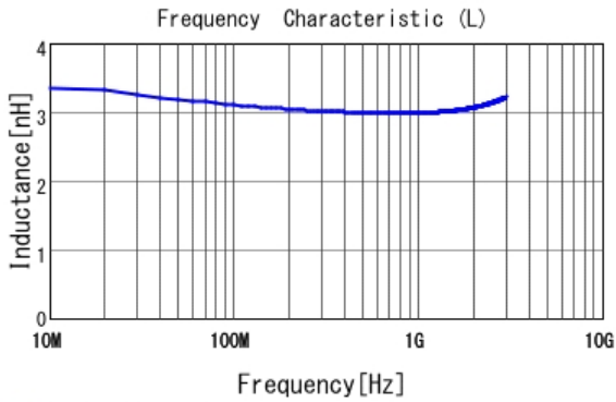
■ LQP03TQ3N0B02 L
