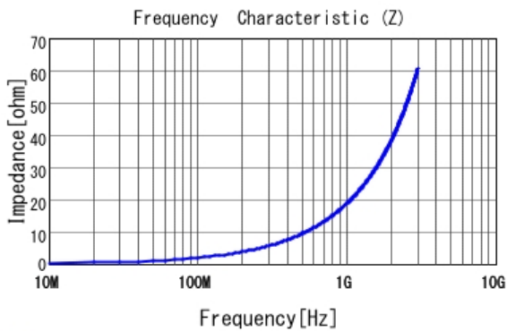
■ LQP03TQ3N0B02 |Z|
