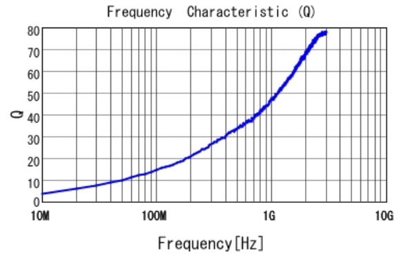
■ LQP03TQ1N9C02 Q
