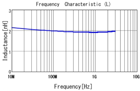
■ LQP03TQ1N9C02 L
