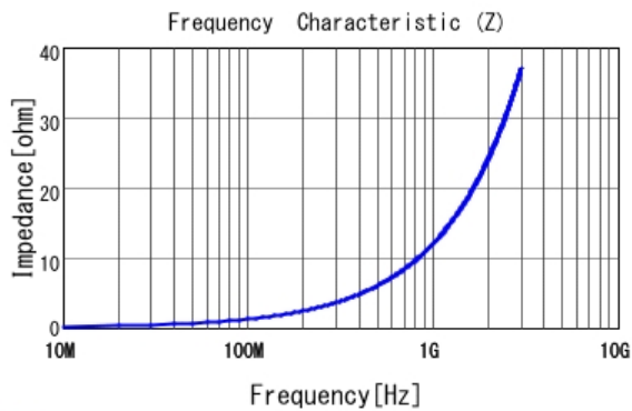
■ LQP03TQ1N9C02 |Z|
