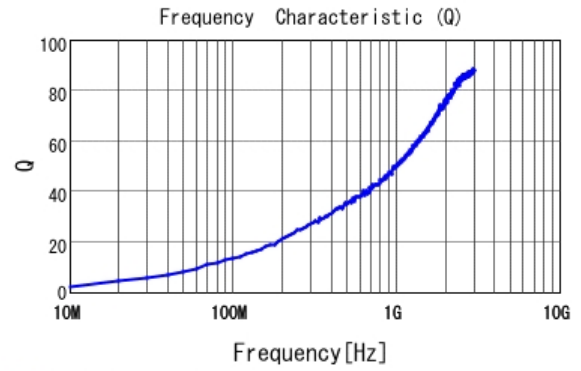
■ LQP03TQ1N5B02 Q
