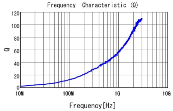
■ LQP03TQ1N1B02 Q
