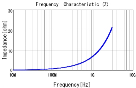
■ LQP03TQ1N1B02 |Z|
