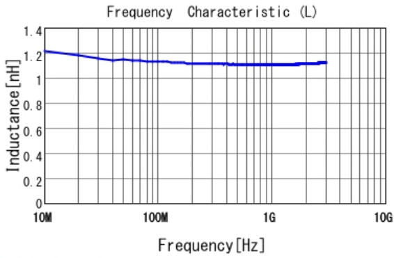
■ LQP03TQ1N1B02 L
