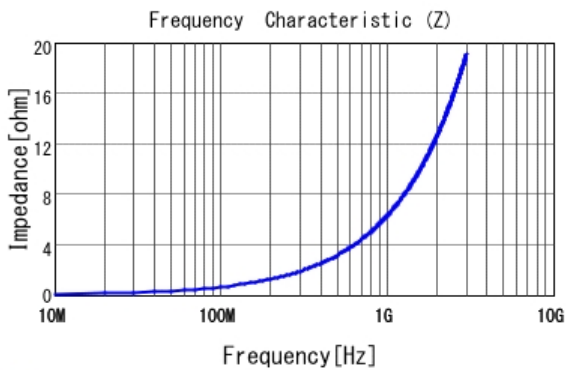
■ LQP03TQ1N0B02 |Z|
