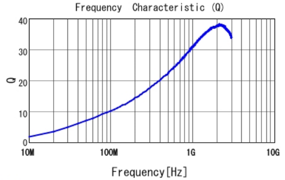
■ LQP03TQ10NJ02 Q
