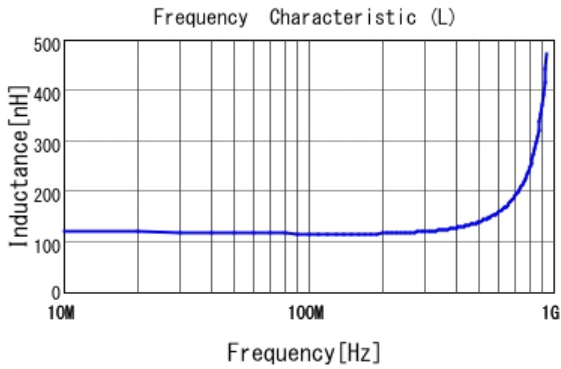
■ LQP03TNR12J02 L
