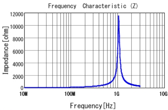
■ LQP03TNR12J02 |Z|
