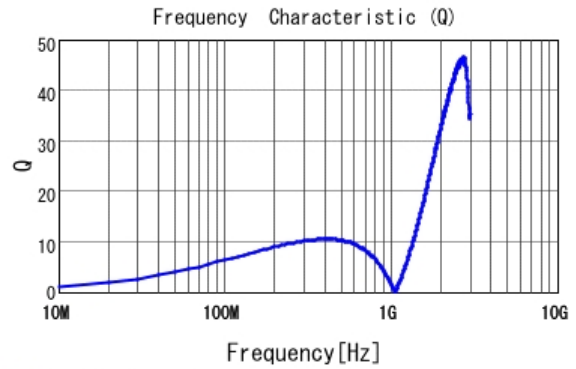
■ LQP03TNR12J02 Q
