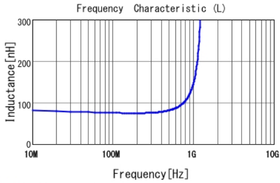
■ LQP03TN75NH02 L
