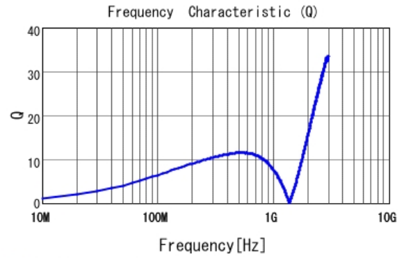
■ LQP03TN75NH02 Q
