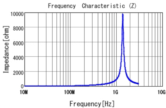
■ LQP03TN75NH02 |Z|
