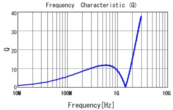
■ LQP03TN68NH02 Q
