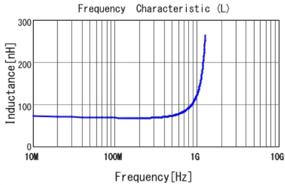
■ LQP03TN68NH02 L
