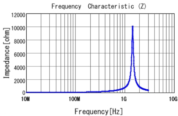
■ LQP03TN68NH02 |Z|
