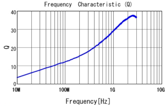
■ LQP03TN5N1J02 Q
