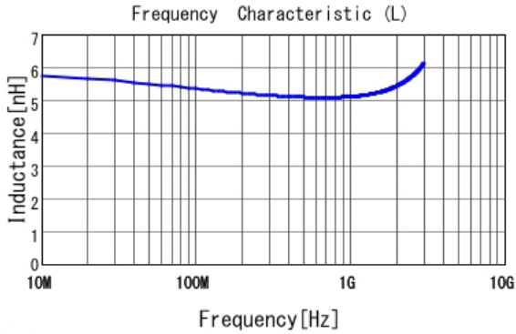
■ LQP03TN5N1J02 L
