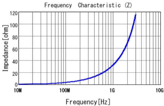
■ LQP03TN5N1J02 |Z|
