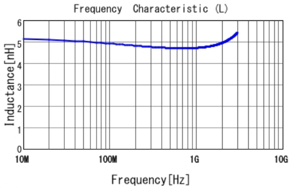
■ LQP03TN4N7J02 L
