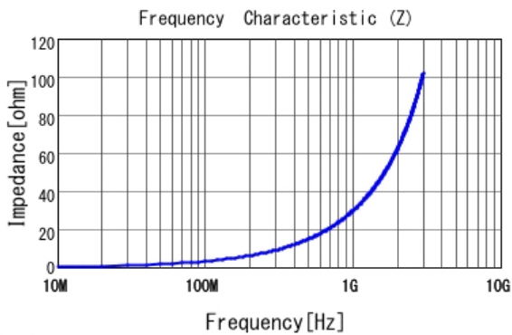
■ LQP03TN4N7J02 |Z|
