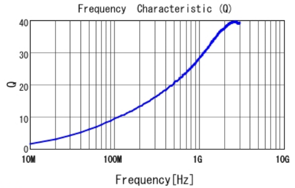
■ LQP03TN4N7J02 Q
