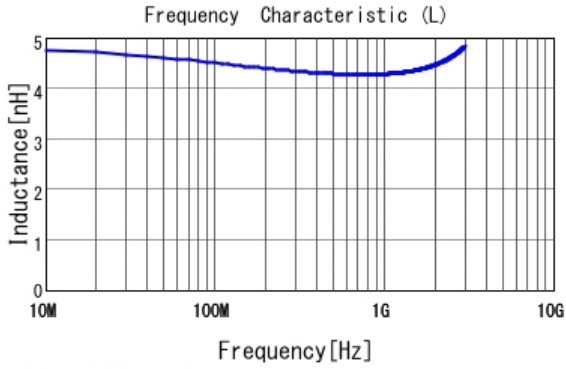
■ LQP03TN4N3J02 L
