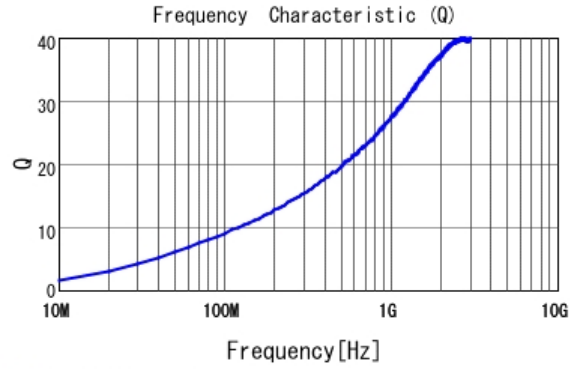
■ LQP03TN4N3J02 Q
