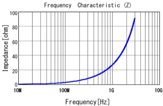
■ LQP03TN4N3J02 |Z|
