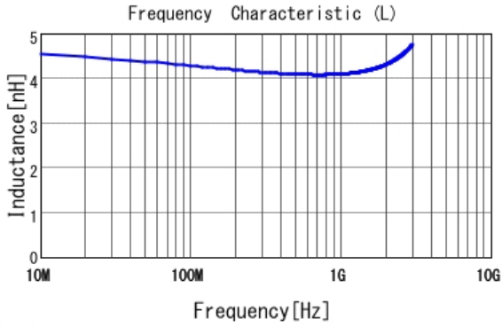
■ LQP03TN4N1B02 L
