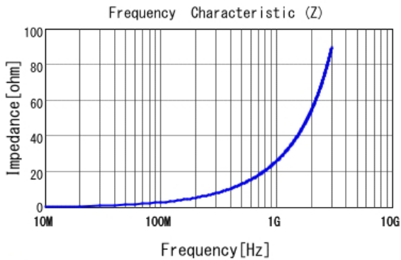
■ LQP03TN4N1B02 |Z|
