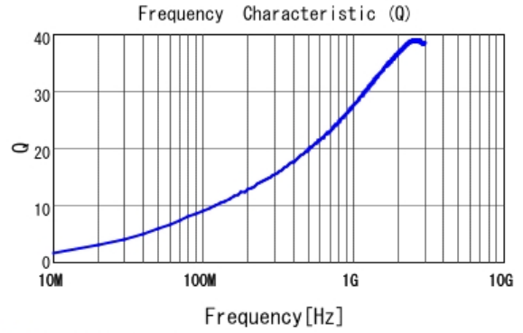
■ LQP03TN4N1B02 Q
